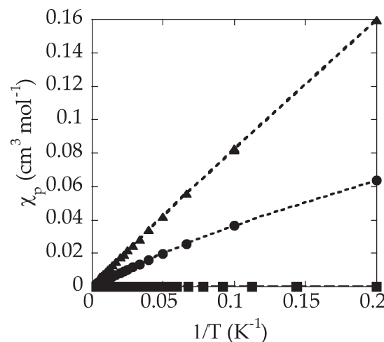
Figure 8. Curie plots for 1 (circles, C = 0.33 \text{ cm}^3 \text{ mol}^{-1} \text{ K} , 1.62 \mu_{\text{B}} ), [1]^+ (squares), and [2]^+ (triangles, C = 0.80 \text{ cm}^3 \text{ mol}^{-1} \text{ K} , 2.53 \mu_{\text{B}} ) collected at 0.1, 0.3, 0.6, and 0.8 T.
