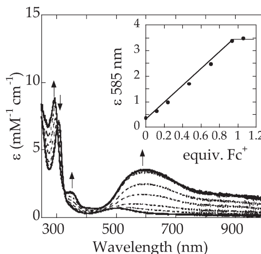
Figure 7. Redox titration of 1 with \text{Fc}^+ in \text{CH}_2\text{Cl}_2 at room temperature (inset: increase in the 585 nm intensity with equivalents of \text{Fc}^+ ).
