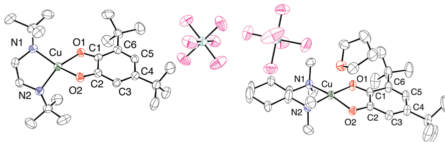
Figure 3. X-ray crystal structures of [1]^+\text{SbF}_6^- (left) and [2]^+\text{SbF}_6^- (right).
