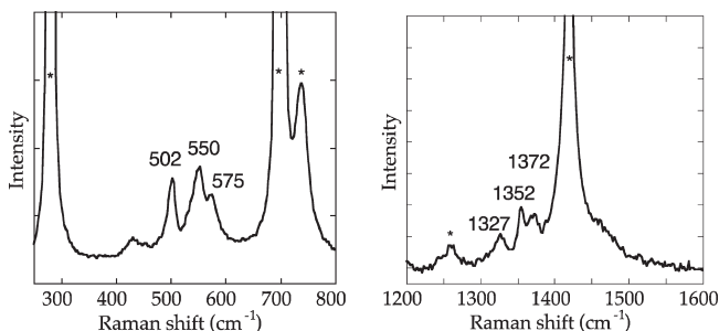
Figure 6. rR spectra of [1]^+ ( \lambda_{\text{ex}} = 530 \text{ nm} , room temperature, \text{CH}_2\text{Cl}_2 ). Solvent features are marked with asterisks.
