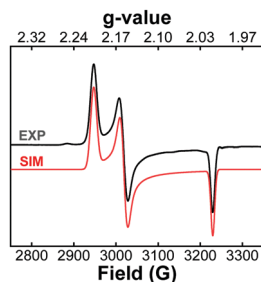
Fig. 8 Experimental (black) and simulated (red) EPR spectra for 1^{2+} after treating it with 1 equiv. of \text{CoCp}_2^* in 1:3 MeCN:PrCN glass at 77 K. The following g values were used for the simulation: g_x = 2.205 , g_y = 2.152 , g_z = 2.012 .
