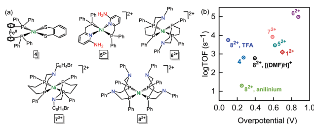
Fig. 7 (a) Selected Ni II HER electrocatalysts reported for efficient HER: 4 , 7 5 2+ , 8 6 2+ , 5a 7 2+ , 5b and 8 2+ . 6a,18 (b) Comparison of the logarithm of TOF vs. the calculated overpotential reported for the Ni electrocatalysts shown in (a) and 1 2+ . The proton sources used are: 0.043 M TFA + 2 M H 2 O in MeCN for 1 2+ , 0.05 M AcOH in THF for 4 , 0.3 M AcOH in MeCN for 5 2+ , 0.42 M [(DMF)H] + + 1.2 M H 2 O in MeCN for 6 2+ , 1.26 M [(DMF)H] + + 1.09 M H 2 O in MeCN for 7 2+ . For 8 2+ , 0.6 M anilinium, 6a 0.25 M [(DMF)H] + , or 1.8 M TFA in MeCN. 18
