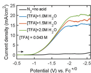
Fig. 6 Linear sweep voltammograms for 1 2+ recorded in N 2 -saturated 0.1 M TBAP/MeCN in the absence of TFA (black) and the presence of 0.043 M TFA + different concentration of H 2 O, 1 M (blue), 1.5 M (orange), and 2.0 M (green). Scan rate = 0.1 V s -1 .
