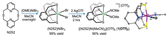
Fig. 2 Synthetic scheme for [(N2S2)Ni(MeCN)2](OTf)_2 ( 1 ) and ORTEP representation (50% probability ellipsoids) for 1^{2+} . Selected bond distances (Å): Ni1–N1 2.071(9), Ni1–N2 2.060(10), Ni1–S1 2.379(3), Ni1–S2 2.394(3), Ni1–N3 2.060(10), Ni1–N4 2.039(10).
