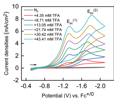
Fig. 3 CVs of 1^{2+} (1 mM) without (black) and with different concentrations of TFA (4.35–43.41 mM) in N 2 -saturated 0.1 M TBAP/MeCN. E_{pc}^{(1)} and E_{pc}^{(2)} indicate the first and second cathodic peak potentials, respectively. Scan rate = 0.1 V s -1 .
