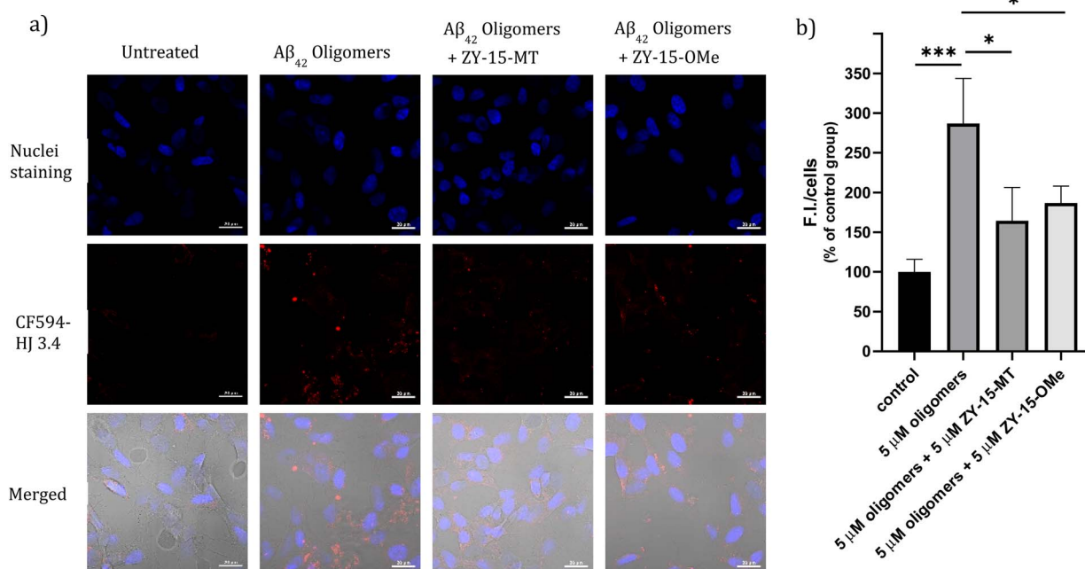
Fig. 10 (a) SH-SY5Y cells were treated with 5 \mu\text{M} A \beta oligomers in the presence or absence of 5 \mu\text{M} ZY-15-MT or 5 \mu\text{M} ZY-15-OMe for 24 h before imaging. Red and blue fluorescence indicate the A \beta oligomers and nuclei, respectively. Scar bar, 20 \mu\text{m} . (b) Three independent experiments were subjected for the statistical analysis and analyzed by one-way ANOVA (* P < 0.05 , *** P < 0.001 ).
