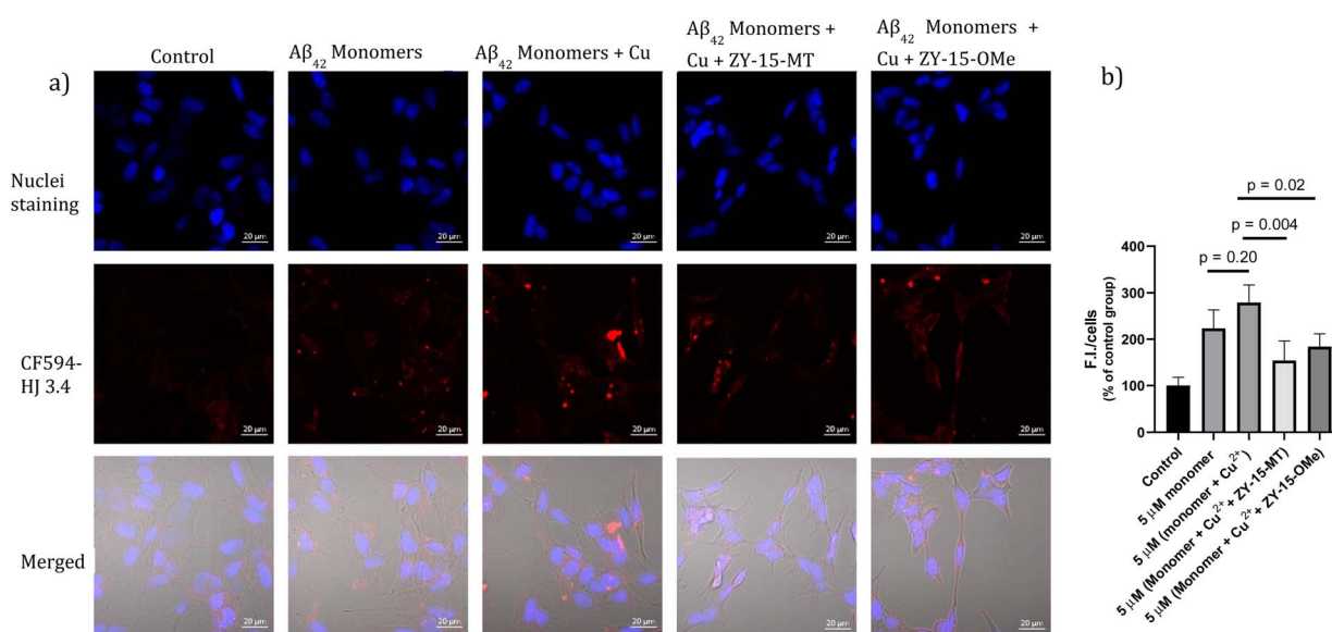
Fig. 11 (a) SH-SY5Y cells were treated with 5 \mu\text{M} A \beta monomers in the presence or absence of 5 \mu\text{M} Cu ^{2+} , 5 \mu\text{M} (Cu ^{2+} + ZY-15-MT) or 5 \mu\text{M} (Cu ^{2+} + ZY-15-OMe) for 48 h before imaging. Red and blue fluorescence indicate the A \beta species and nuclei, respectively. Scar bar, 20 \mu\text{m} . (b) Three independent experiments were subjected for the statistical analysis and analyzed by one-way ANOVA (* P < 0.05 , ** P < 0.01 ).
