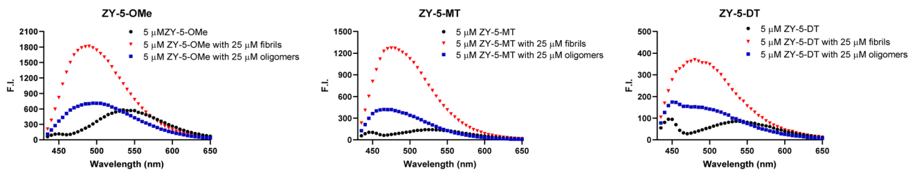
Fig. 2 Fluorescence turn-on effects with Aβ 42 oligomers and fibrils. Left ZY-5-OMe, middle ZY-5-MT right ZY-5-DT. Black: compound only; Blue: compound + Aβ 42 oligomers; Red: compound + Aβ 42 fibrils; [compound] = 5 μM; [Aβ 42 oligomers] = 25 μM; [Aβ 42 fibrils] = 25 μM.
