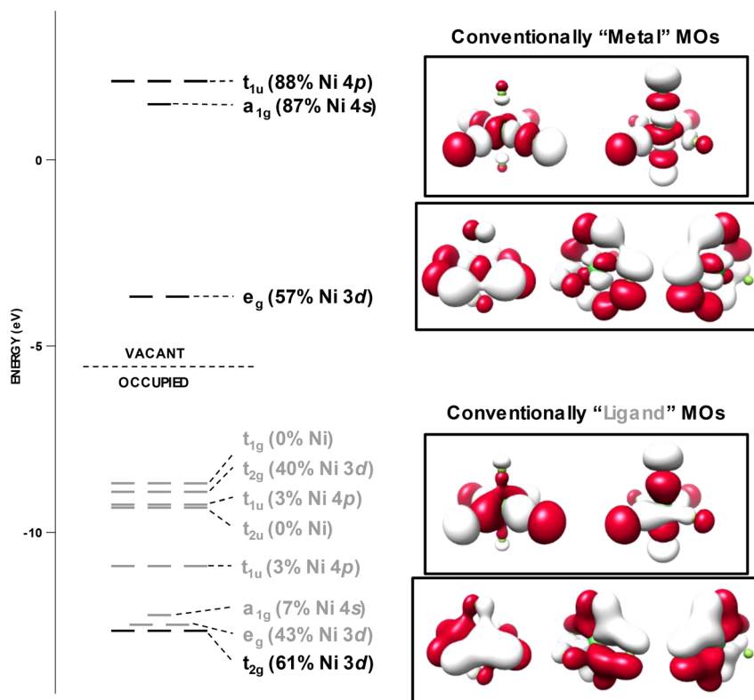
Fig. 10 Frontier MO diagram for NiF 6 2- calculated at the B3LYP/CP(PPP)/ZORA-def2-TZVP(-f) level. Predominantly metal-based orbitals are black, ligand-based orbitals are grey. Orbitals are plotted at an isovalue of 0.03 au.
