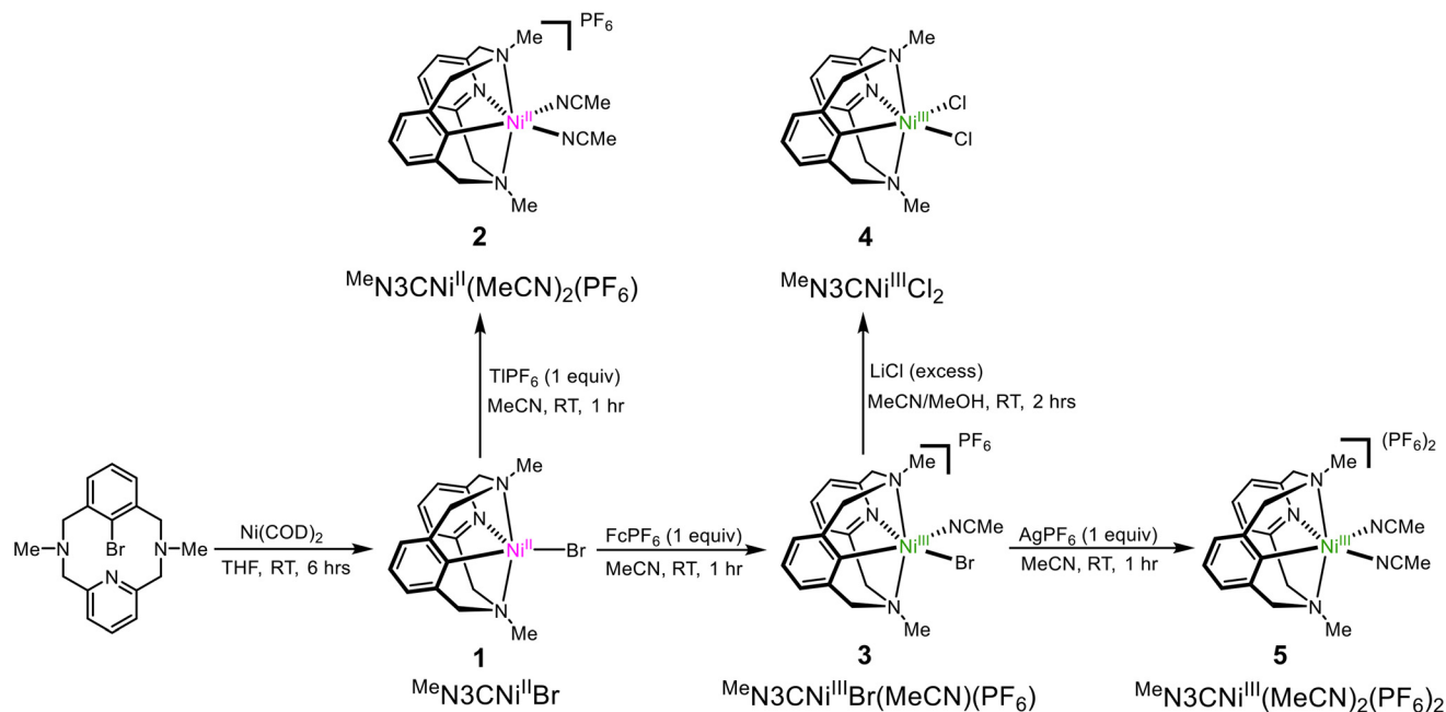
Scheme 1 Synthesis of ( Me N 3 C)Ni complexes.
